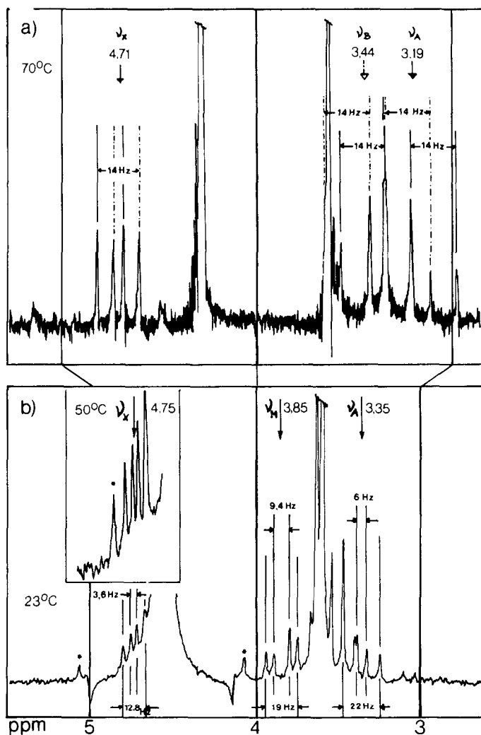
FIG. 2. ^1\text{H} -nmr spectra of cysteine and glutathione substitution products. (a) After rearrangement to the 2- N -alkylpyrimidine 5a an ABX -type spectrum is obtained. (b) The glutathione product 11 gives an S -alkylpyrimidine AMX -type spectrum. For details see text and Table 1.
