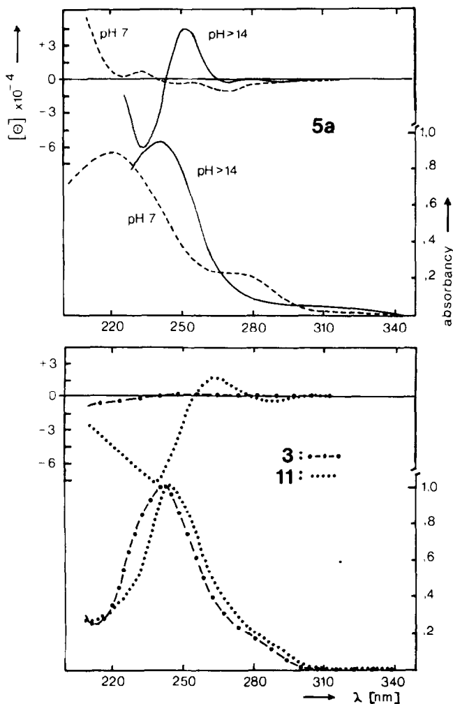
FIG. 1. uv and CD spectra of 1-methylpyrimidines 5a , 3 , and 11 . The CD spectrometer was not capable of measuring below 210 nm.
