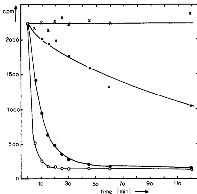
FIG. 3. Decay of ^{14}\text{C} -radioactivity during the reaction of \text{tRNA}^{\text{Phe}}\text{-C}_{74}\text{-}([^{14}\text{C}]\text{IAA})\text{s}^2\text{C}_{75}\text{-A}_{76} with lysine at pH 9.0 (■), cysteine at pH 7.0 (●), and pH 9.0 (○), control (×) at 37^\circ\text{C} (for details see text).
